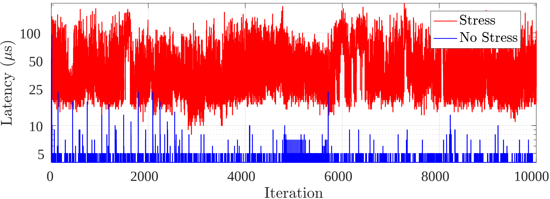
Latency for Scheduler: SCHED_DEADLINE R800
